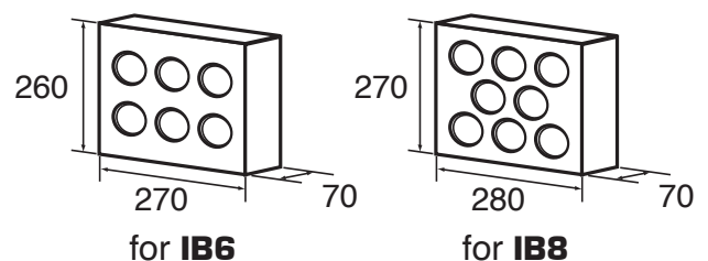
Material Ice Plate for Ø65 (mm)
